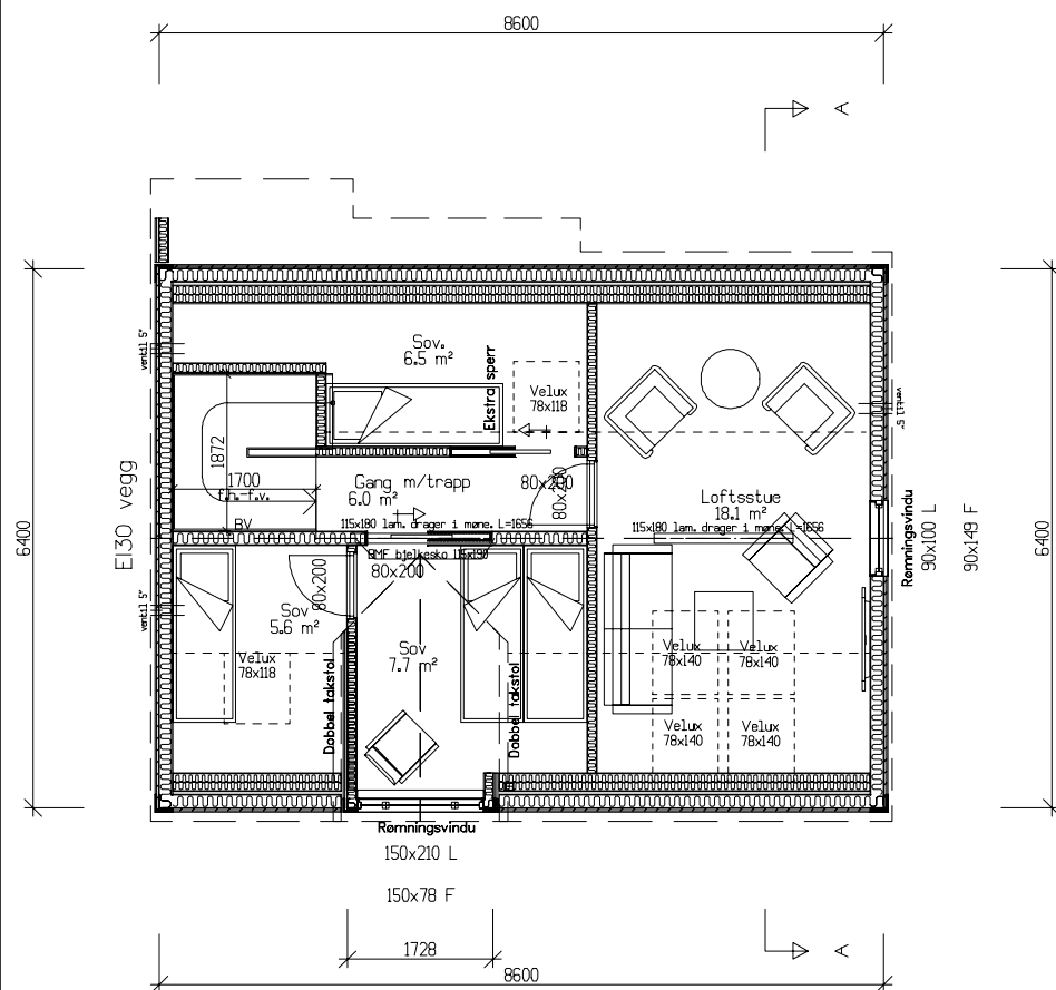
Loftsplan Bra=35,1m 2
