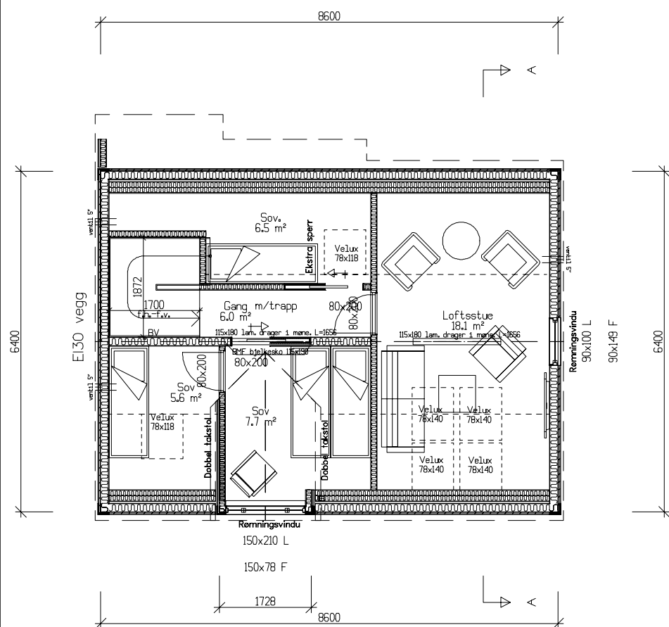
Loftsplan Bra=35,1m 2
