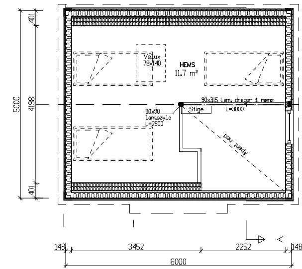
Hems Bra=11,7m 2
